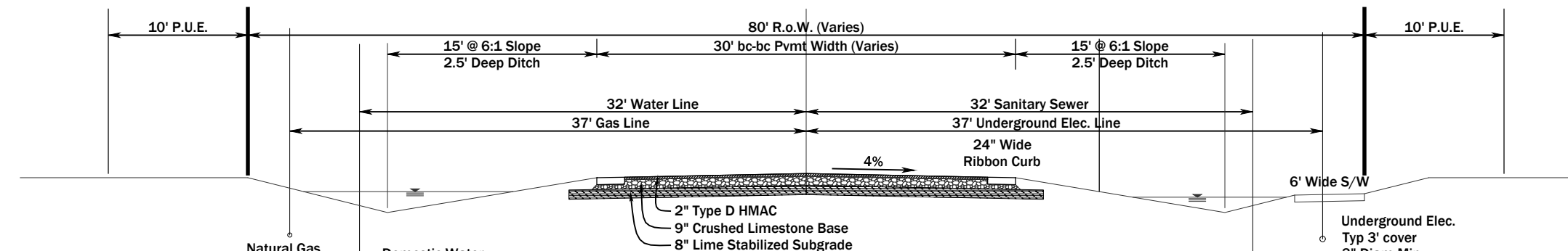
Typical Collector Roadway Section w/ Utility Assignments N.T.S.
